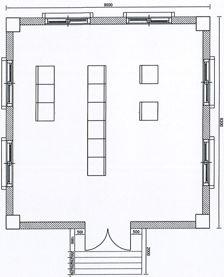
GROUND FLOOR PLAN OF 230KV SPR BUILDING
